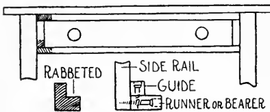
FIG. 427. DRAWER RUNNERS AND GUIDES CHEAP CONSTRUCTION.
